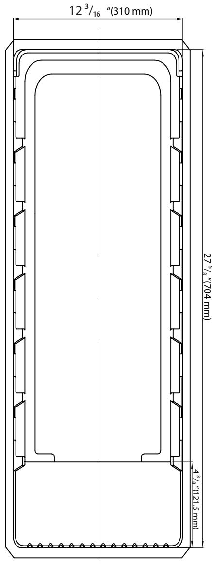
Front View
