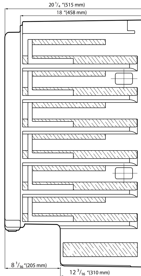
Side View
